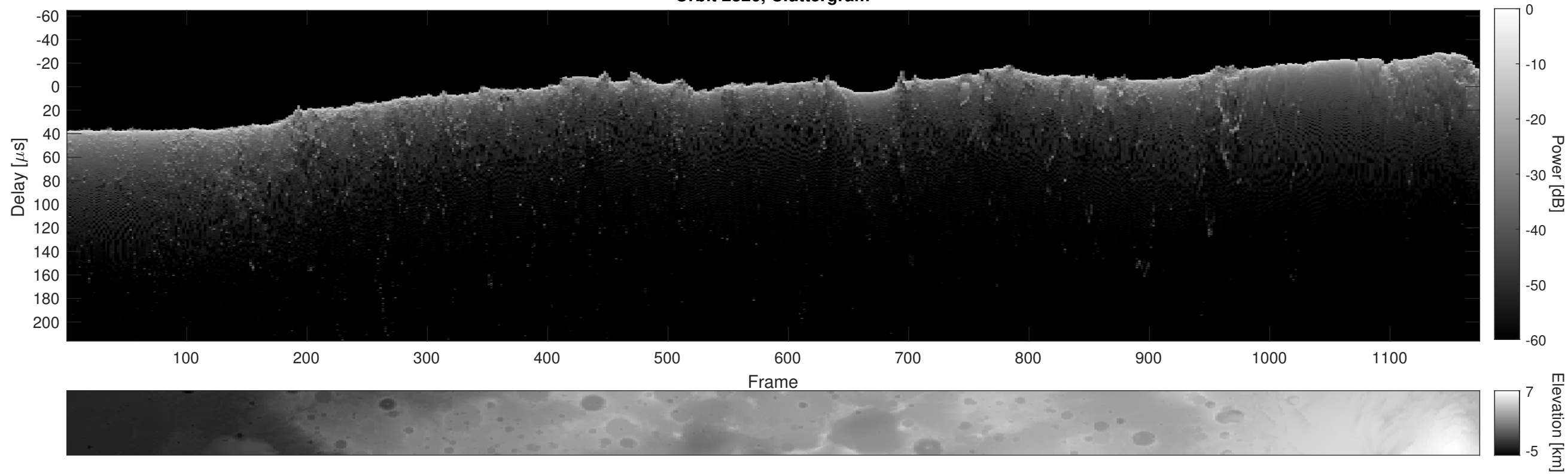
Orbit 2826, Cluttergram
