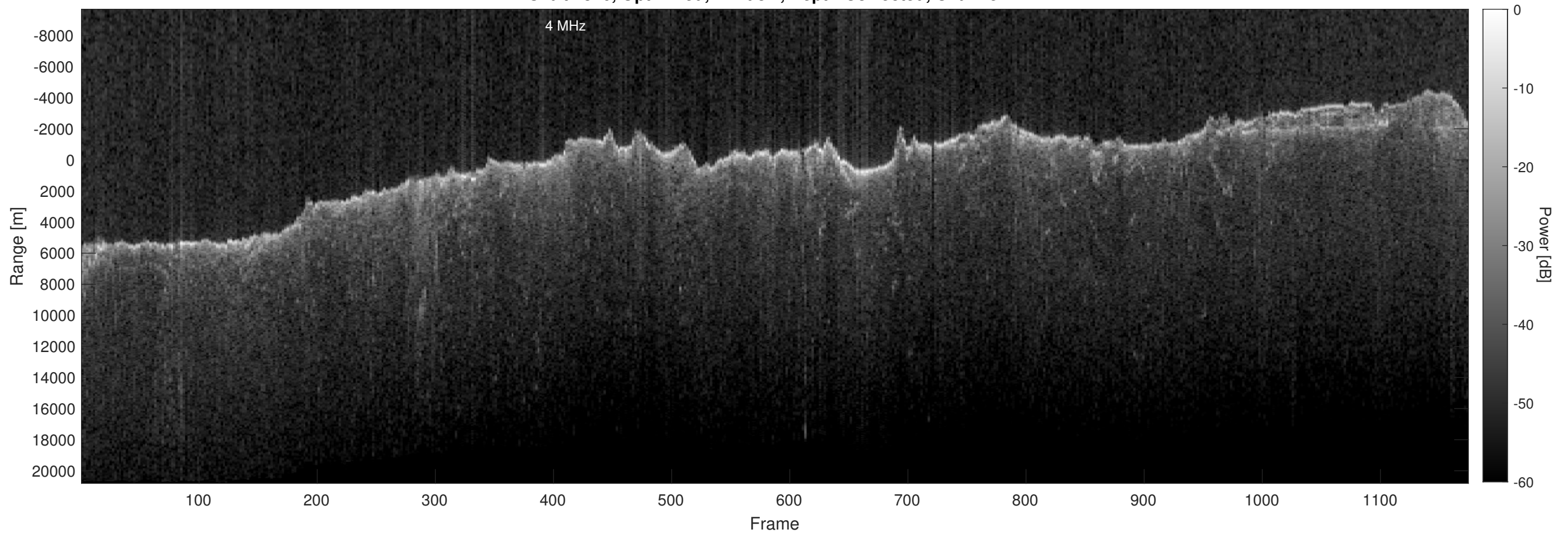
Orbit 2826, Optimized, Window, Depth-Corrected, Channel 2
