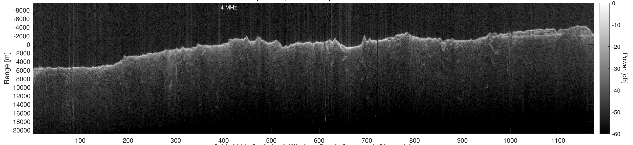
Orbit 2826, Optimized, Window, Depth-Corrected, Channel 2
