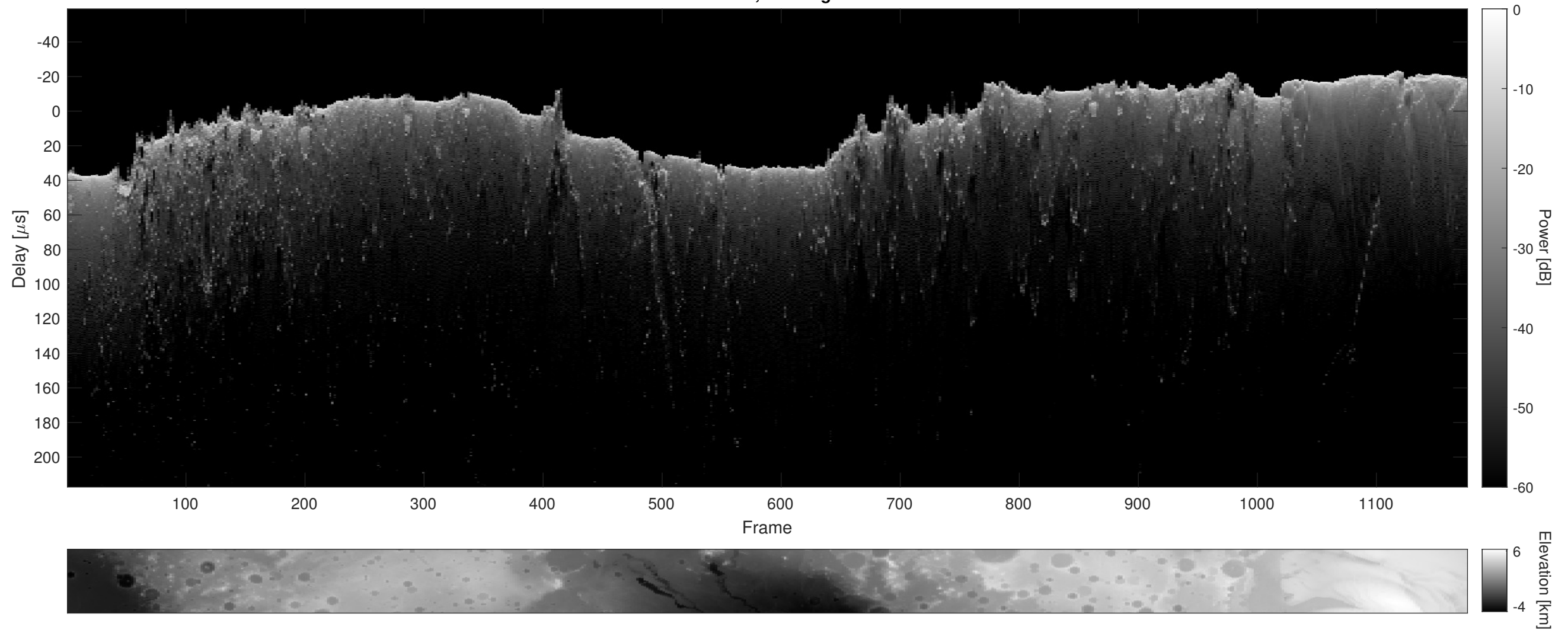
Orbit 2827, Cluttergram
