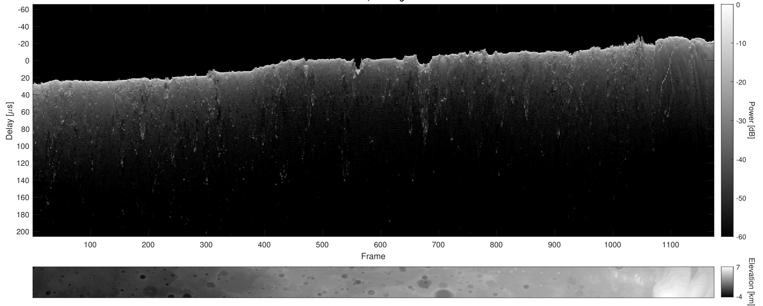
Orbit 2828, Cluttergram
