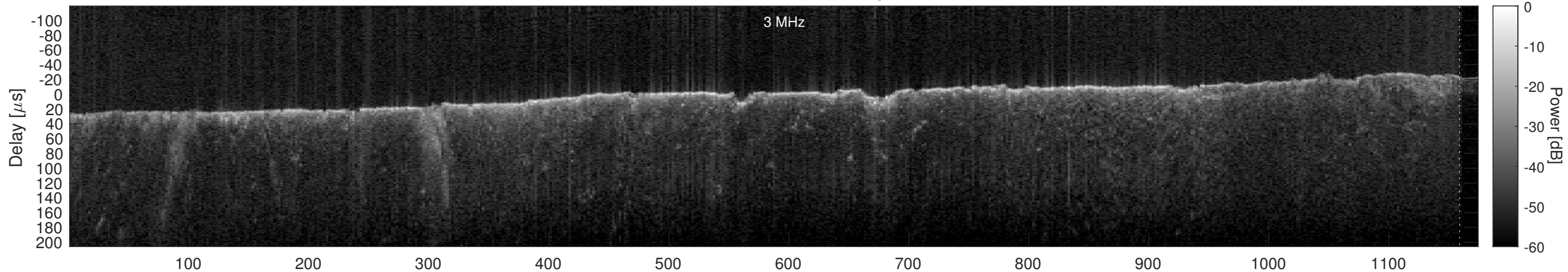
Orbit 2828, Cluttergram
