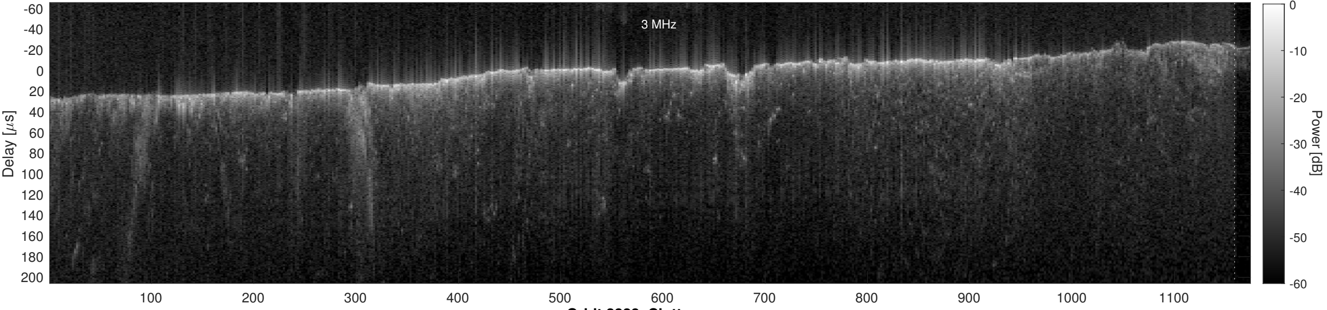
Orbit 2828, Cluttergram
