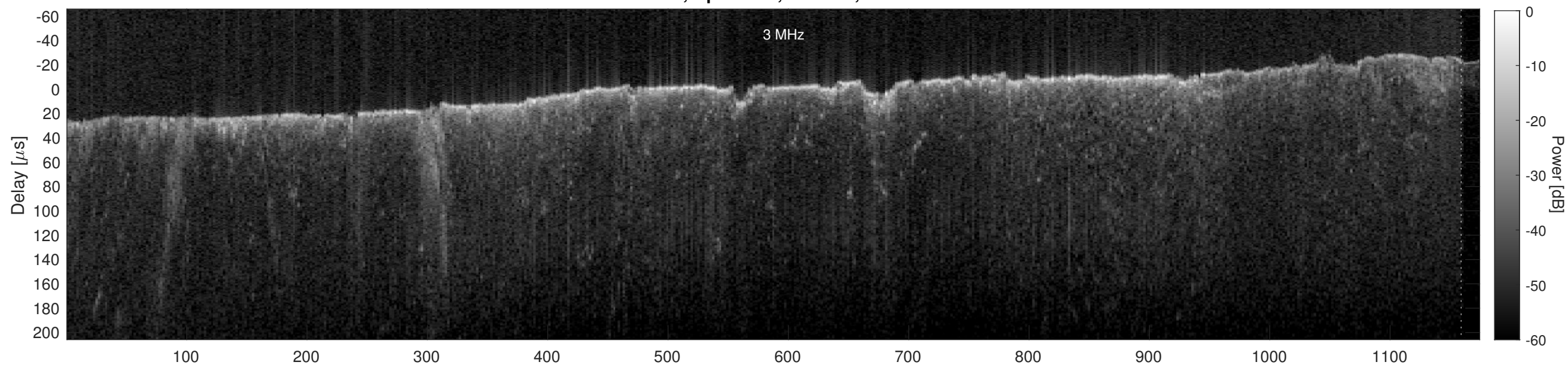
Orbit 2828, Cluttergram
