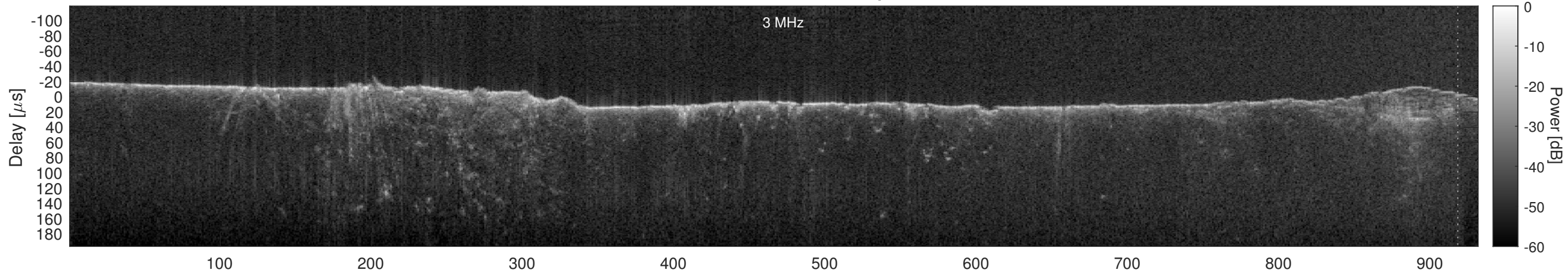
Orbit 2829, Cluttergram
