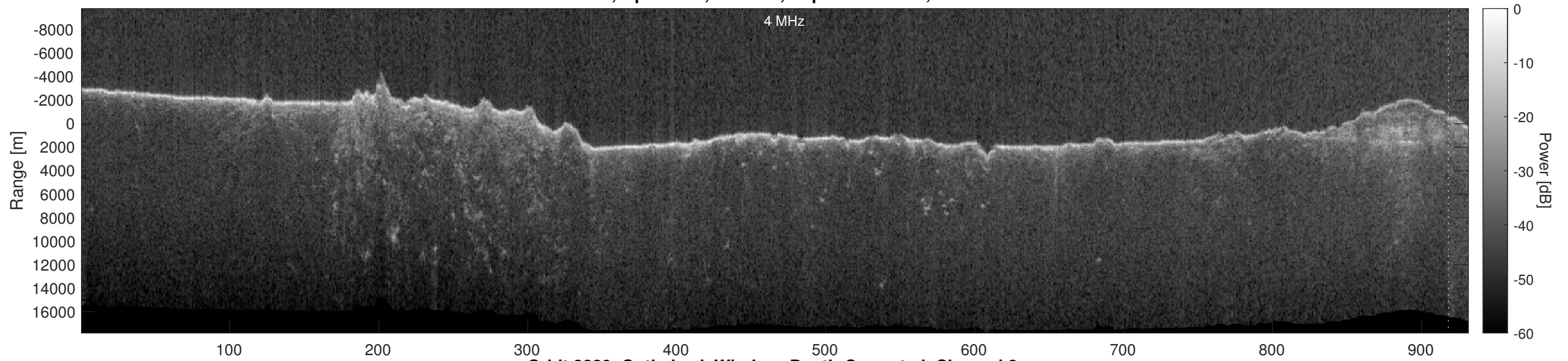
Orbit 2829, Optimized, Window, Depth-Corrected, Channel 2
