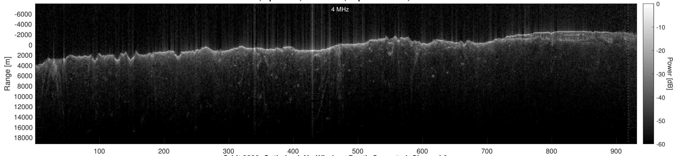
Orbit 2830, Optimized, No Window, Depth-Corrected, Channel 2
