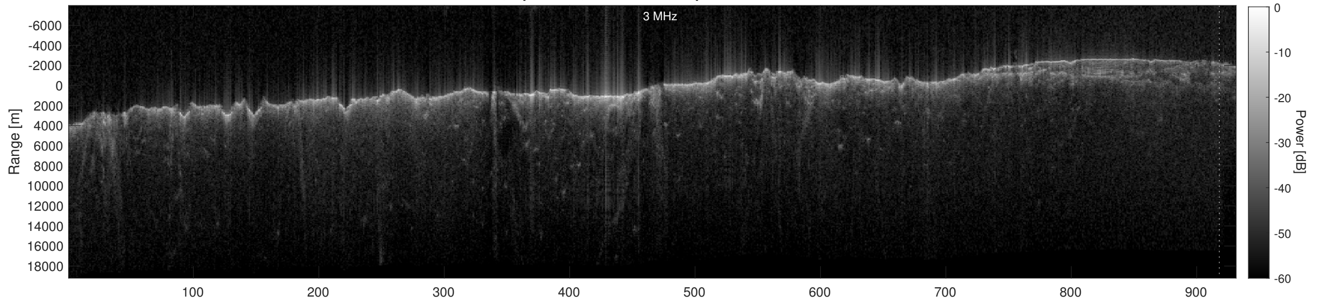
Orbit 2830, Depth-Corrected Cluttergram
