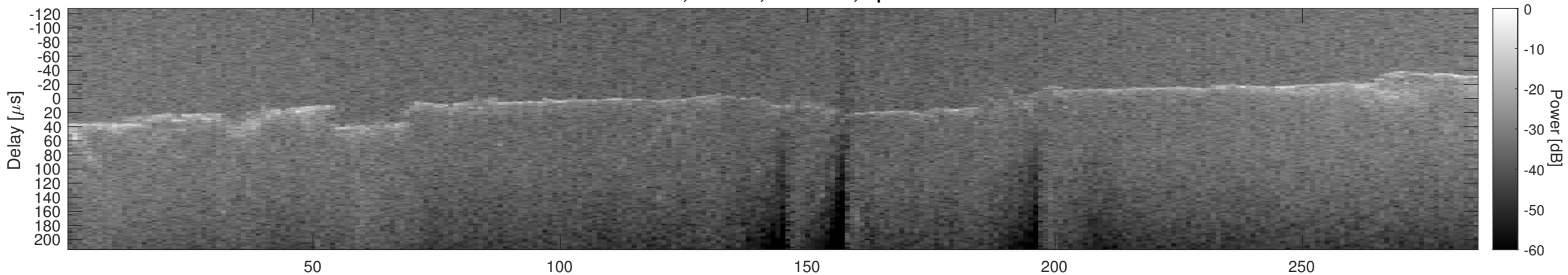
Orbit 2832, Cluttergram
