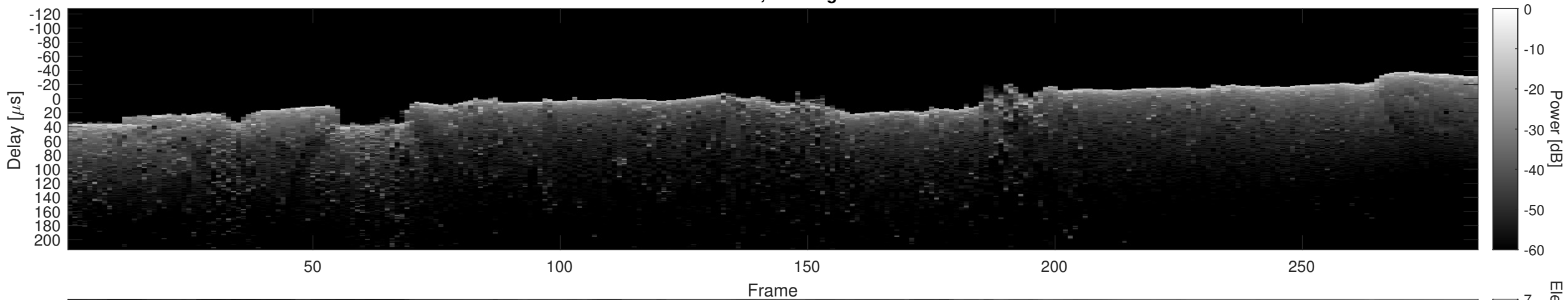
Orbit 2832, Cluttergram
