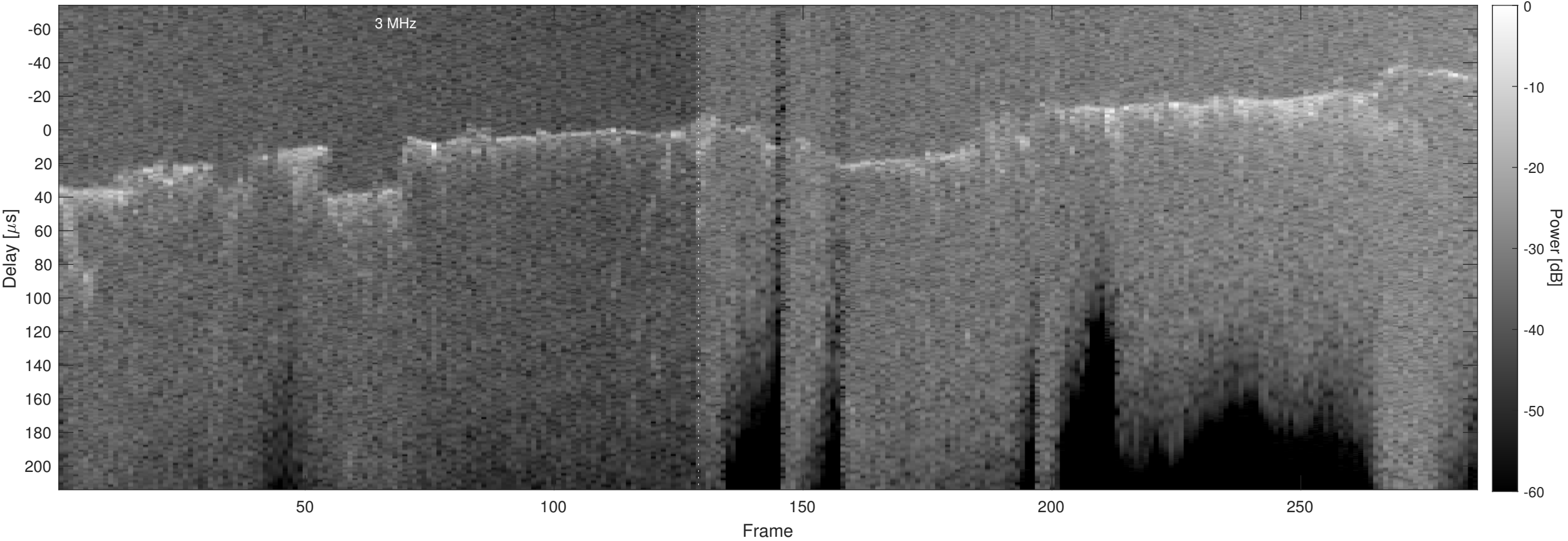
Orbit 2832, Optimized, Window, Channel 2
