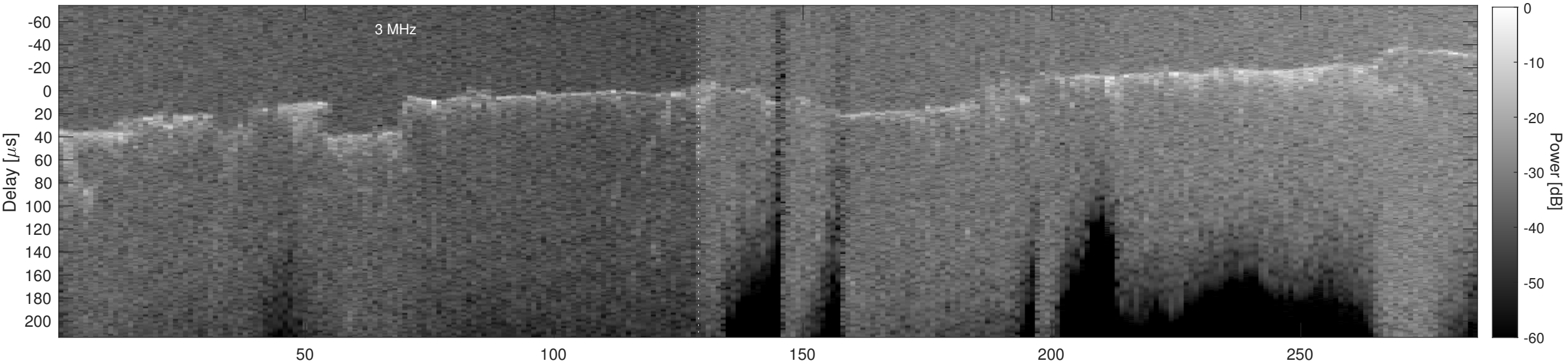
Orbit 2832, Cluttergram
