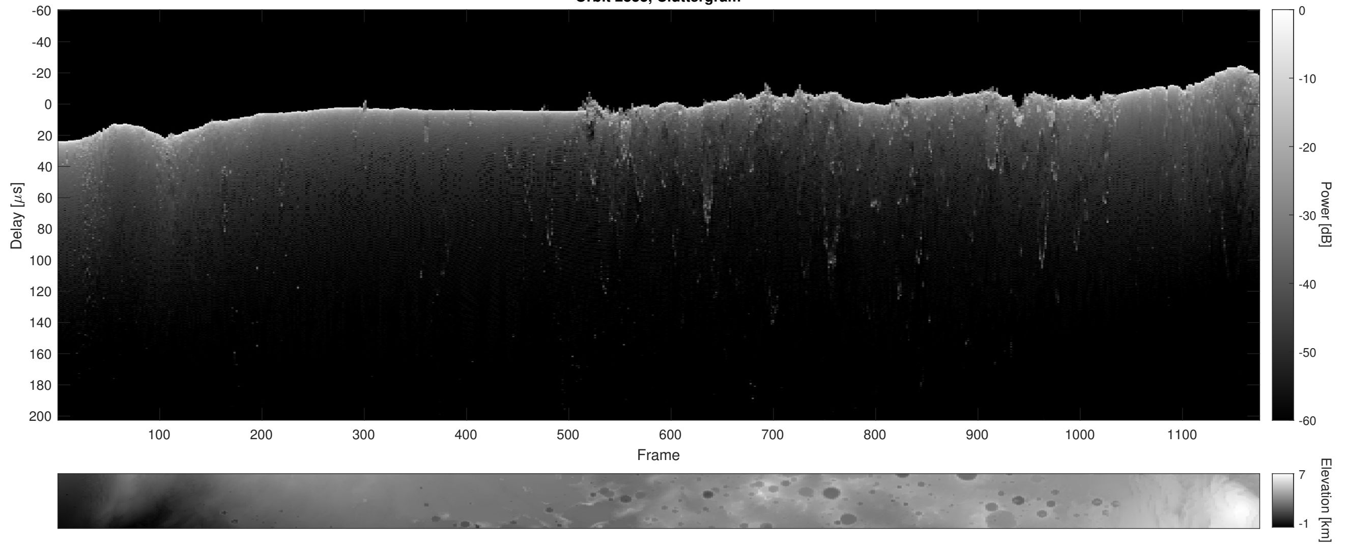
Orbit 2833, Cluttergram
