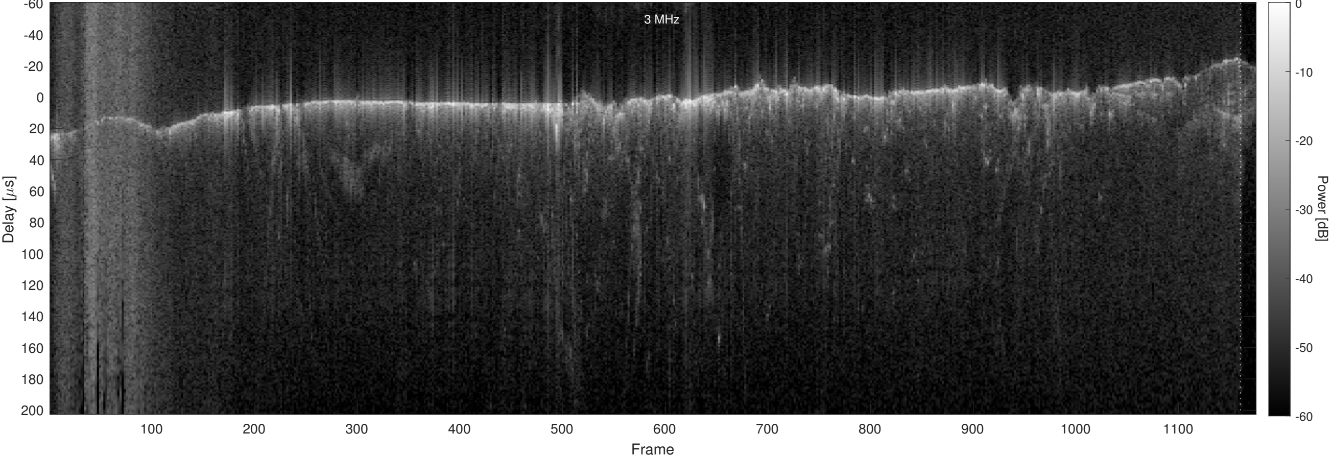
Orbit 2833, Optimized, No Window, Channel 2
