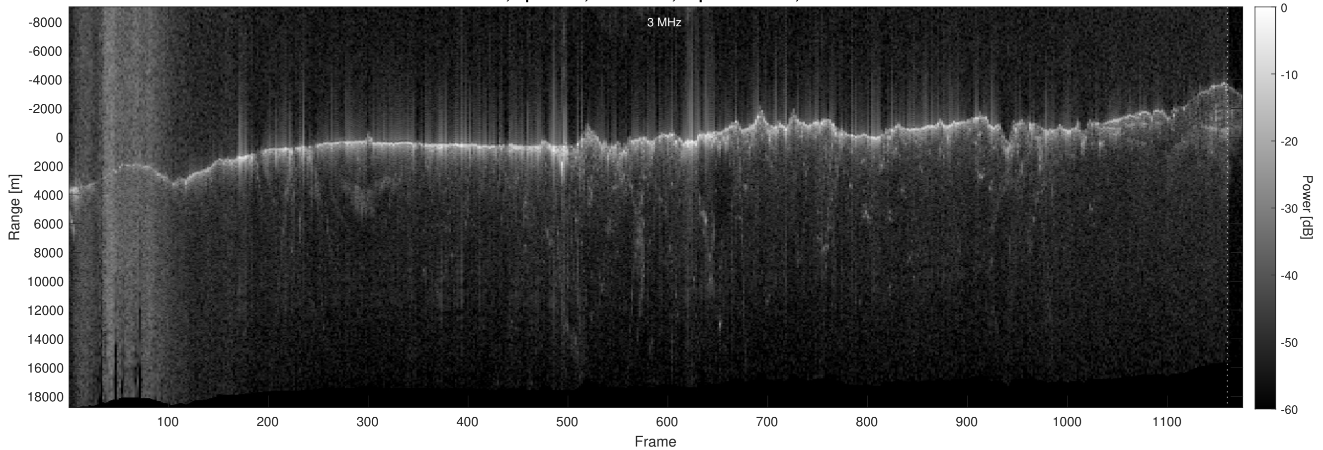
Orbit 2833, Optimized, No Window, Depth-Corrected, Channel 2
