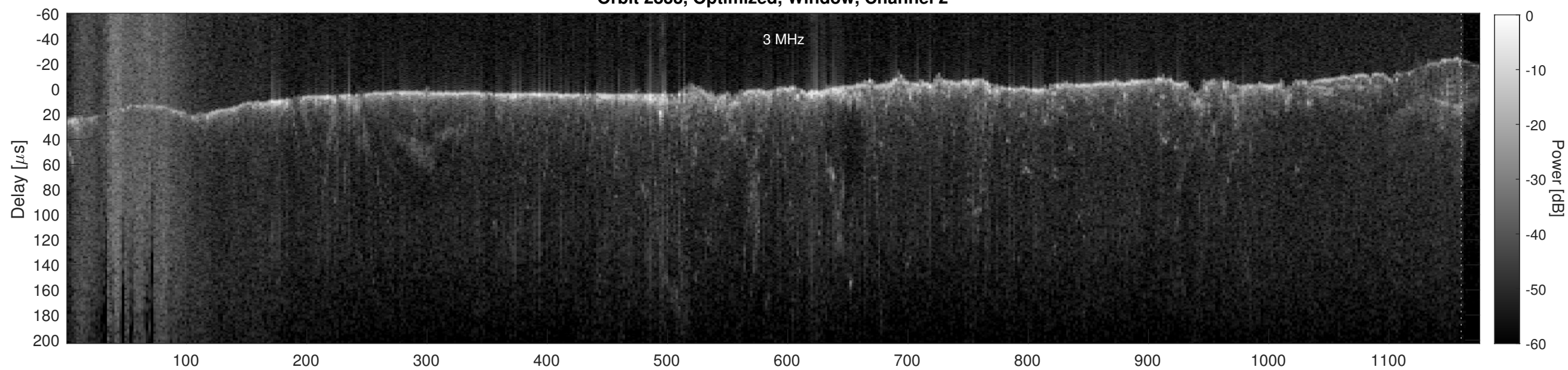
Orbit 2833, Cluttergram
