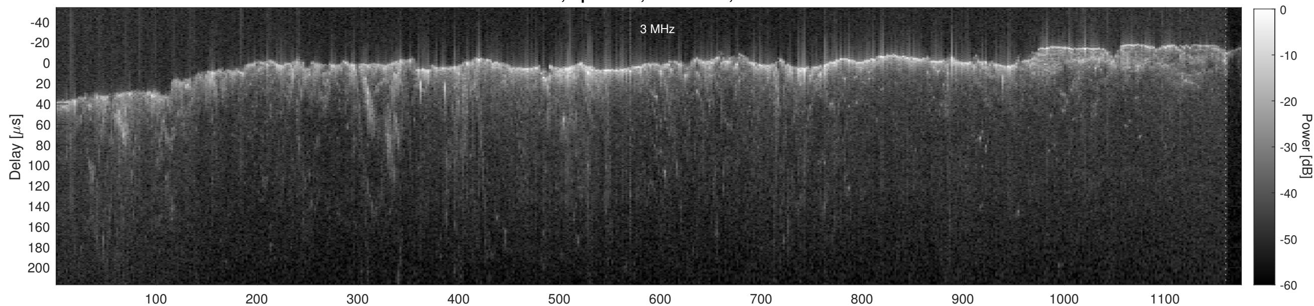
Orbit 2834, Cluttergram
