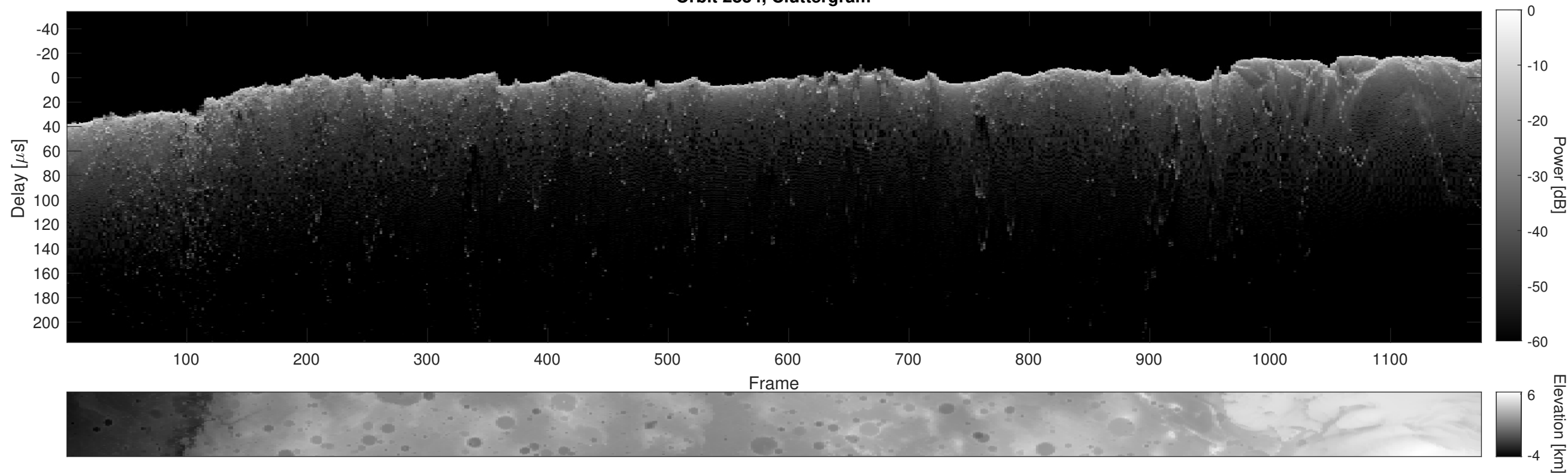
Orbit 2834, Cluttergram
