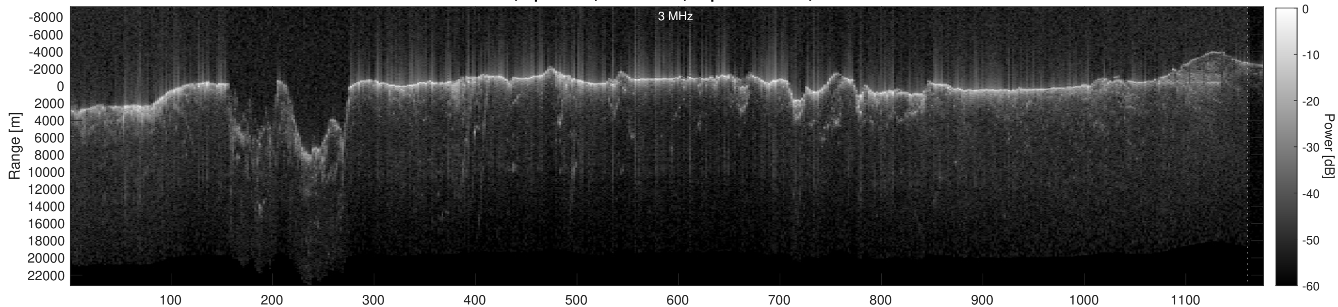
Orbit 2836, Depth-Corrected Cluttergram
