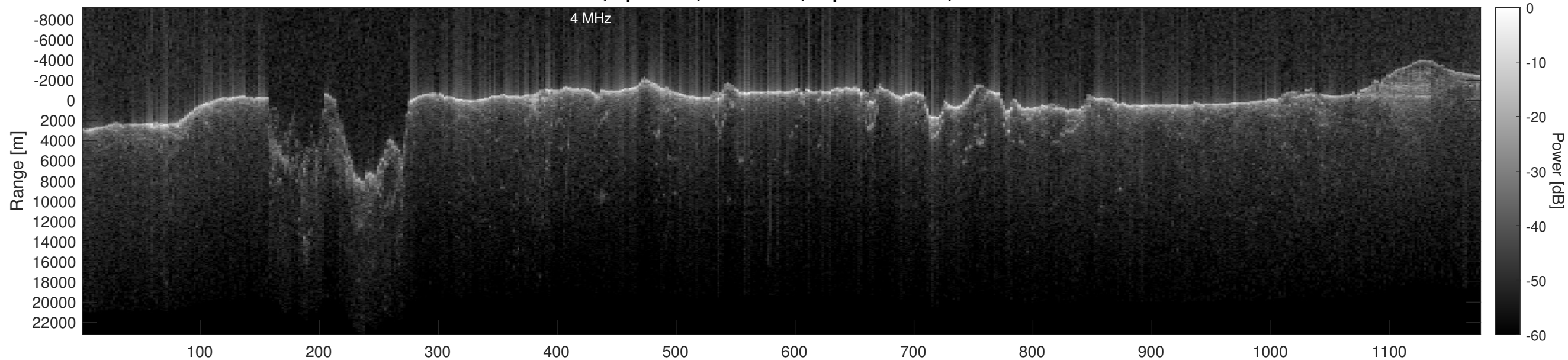
Orbit 2836, Optimized, No Window, Depth-Corrected, Channel 2
