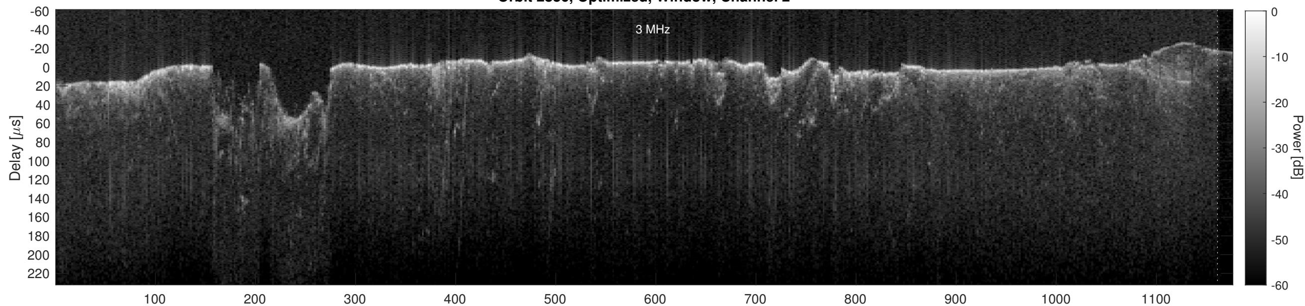
Orbit 2836, Cluttergram
