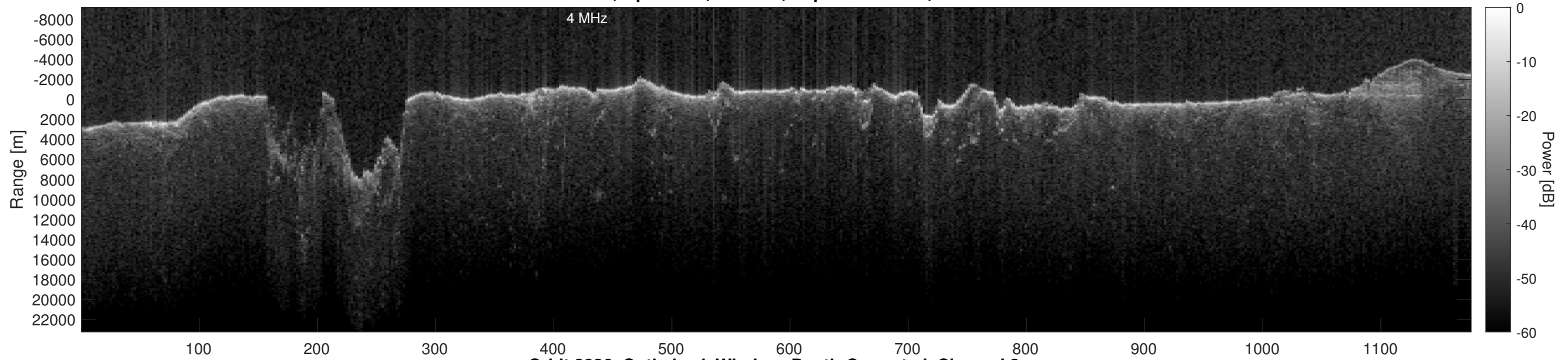
Orbit 2836, Optimized, Window, Depth-Corrected, Channel 2
