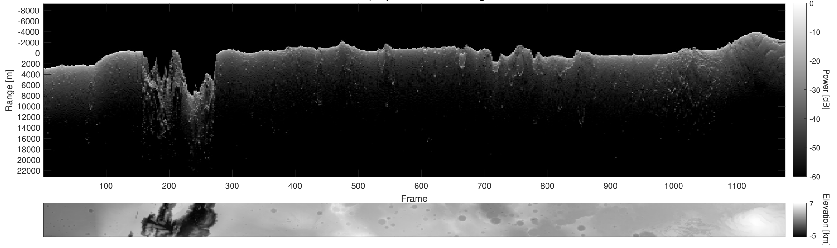
Orbit 2836, Depth-Corrected Cluttergram
