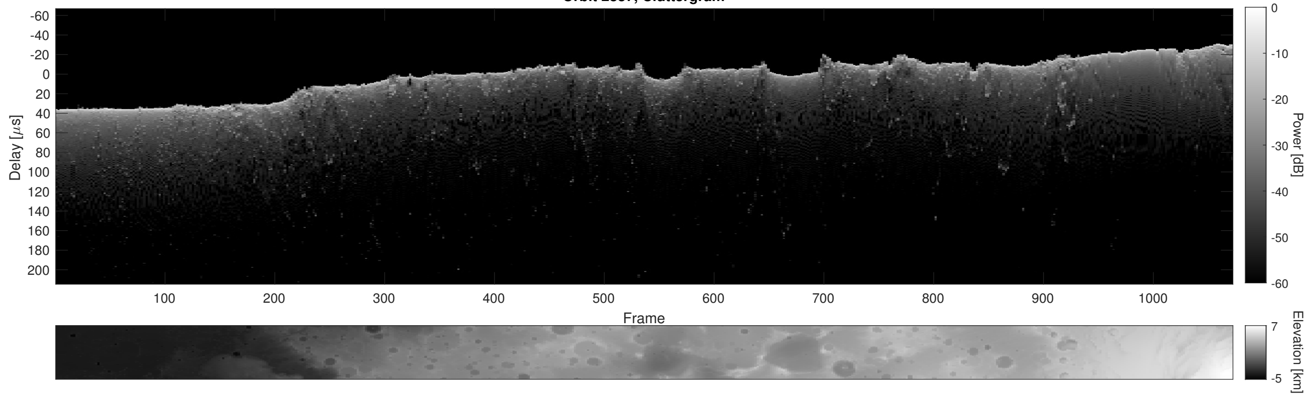
Orbit 2837, Cluttergram
