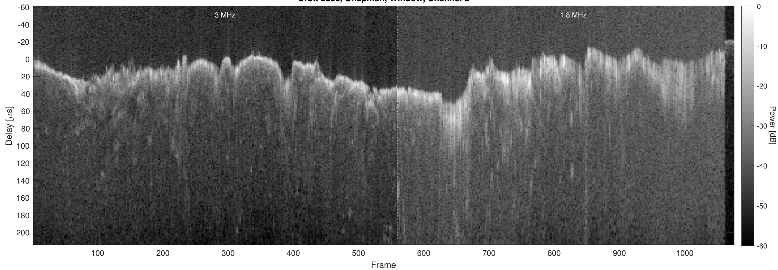
Orbit 2838, Chapman, Window, Channel 2
