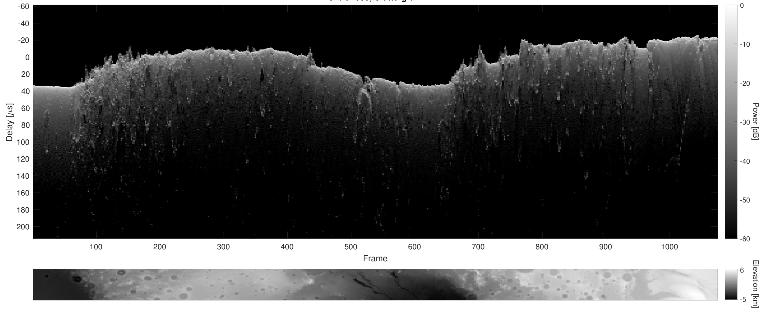
Orbit 2838, Cluttergram
