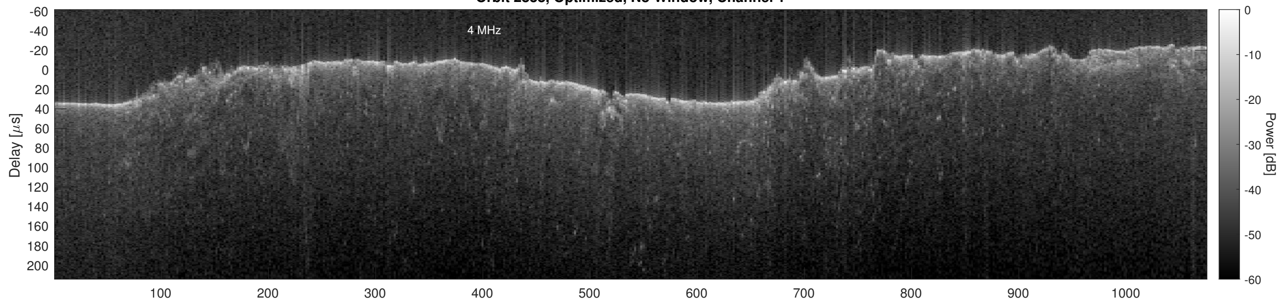
Orbit 2838, Optimized, No Window, Channel 2
