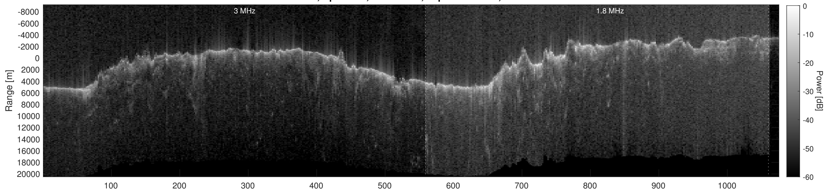
Orbit 2838, Depth-Corrected Cluttergram
