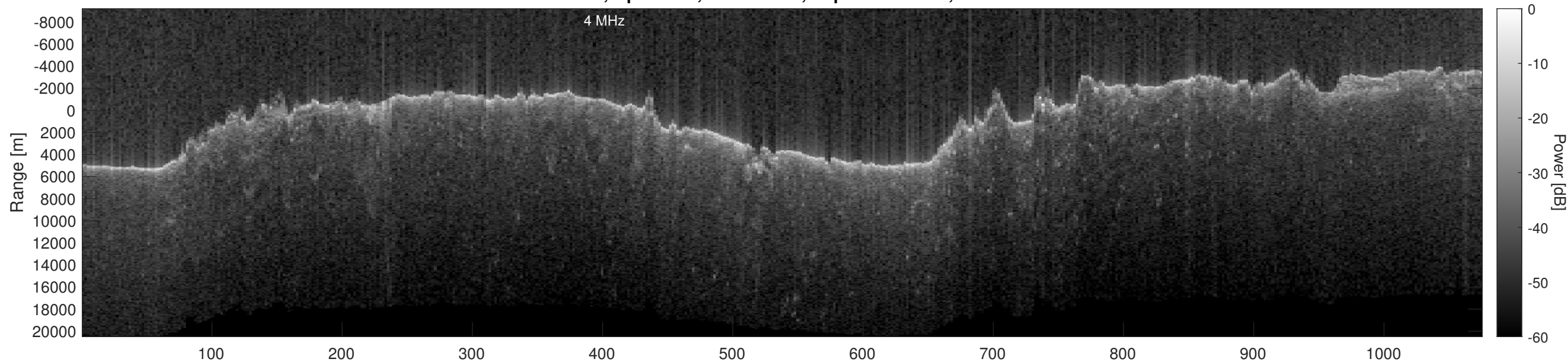
Orbit 2838, Optimized, No Window, Depth-Corrected, Channel 2
