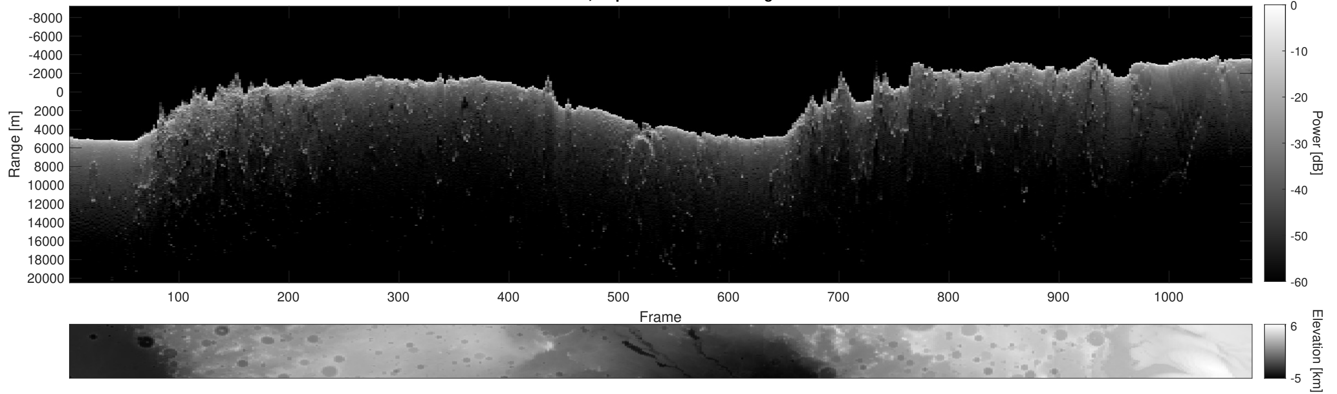
Orbit 2838, Depth-Corrected Cluttergram
