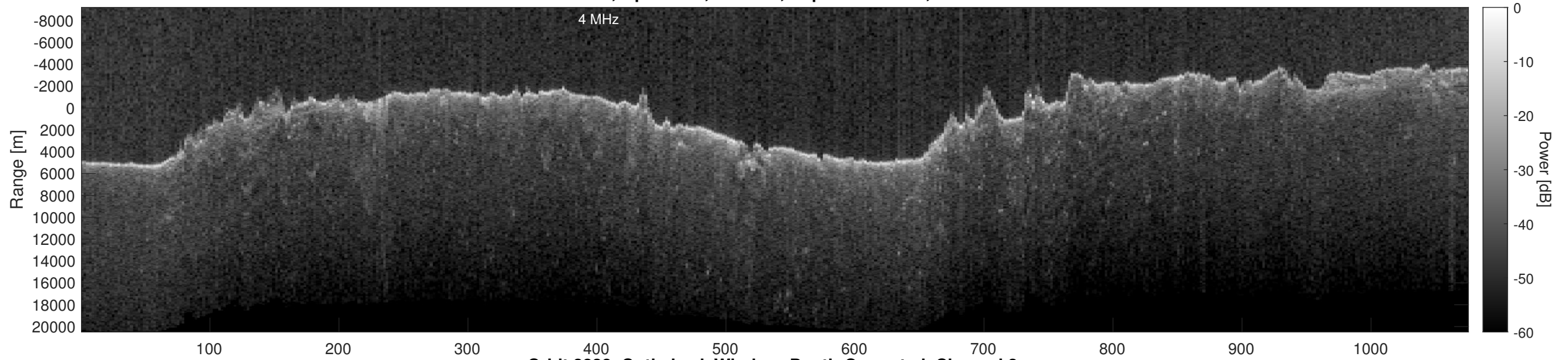
Orbit 2838, Optimized, Window, Depth-Corrected, Channel 2
