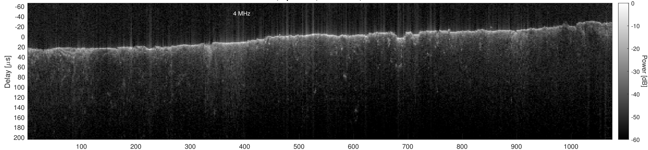
Orbit 2839, Optimized, No Window, Channel 2
