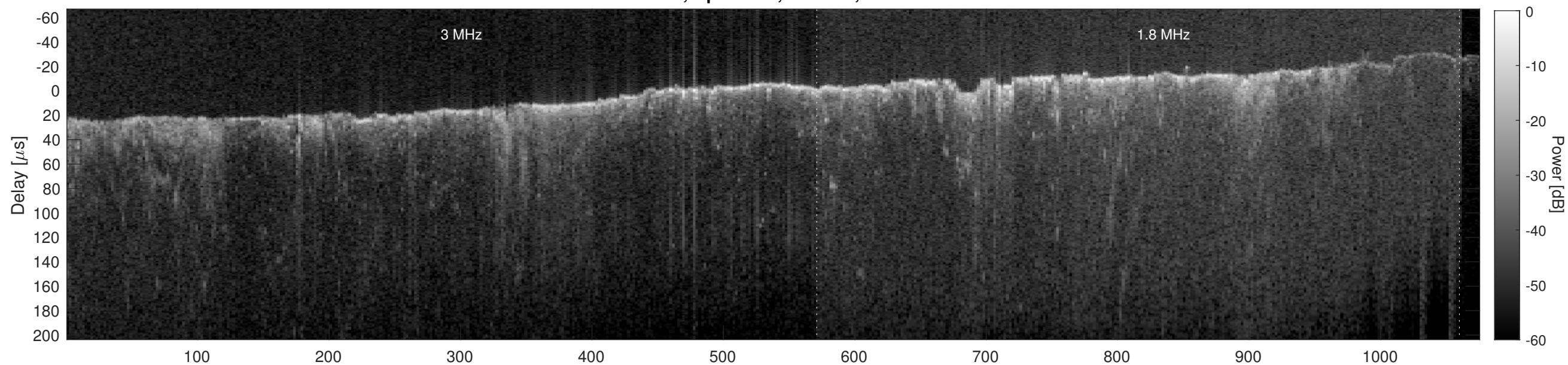
Orbit 2839, Cluttergram
