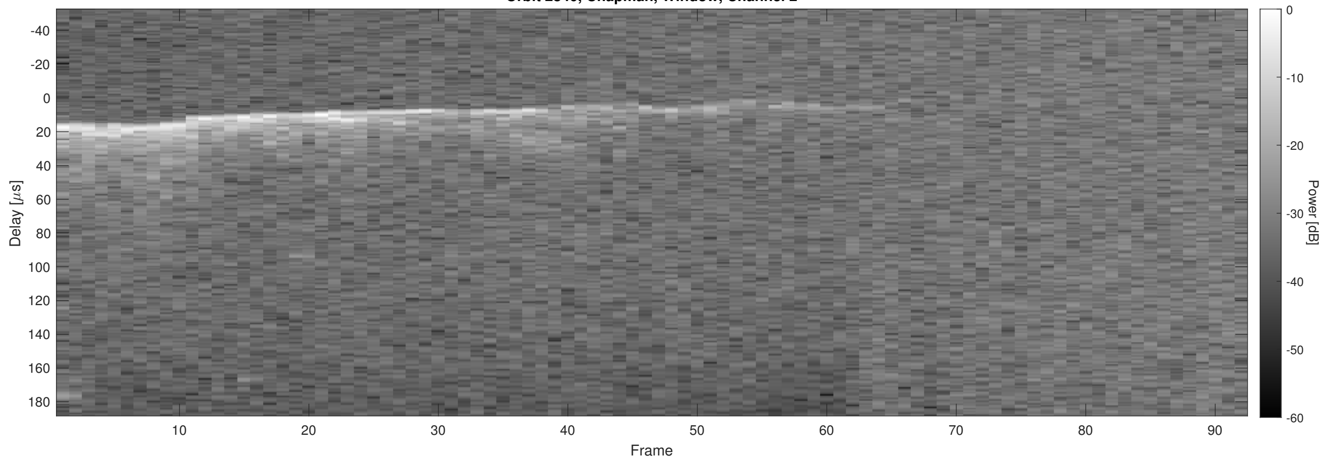
Orbit 2840, Chapman, Window, Channel 2
