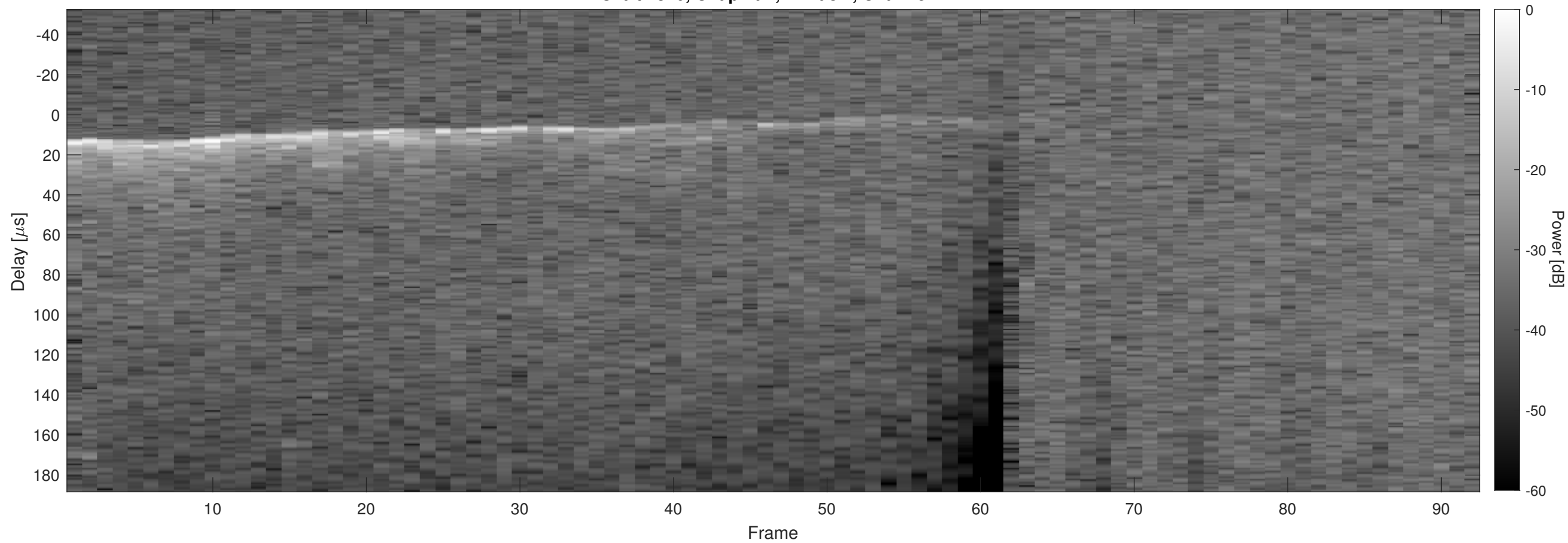
Orbit 2840, Chapman, Window, Channel 2
