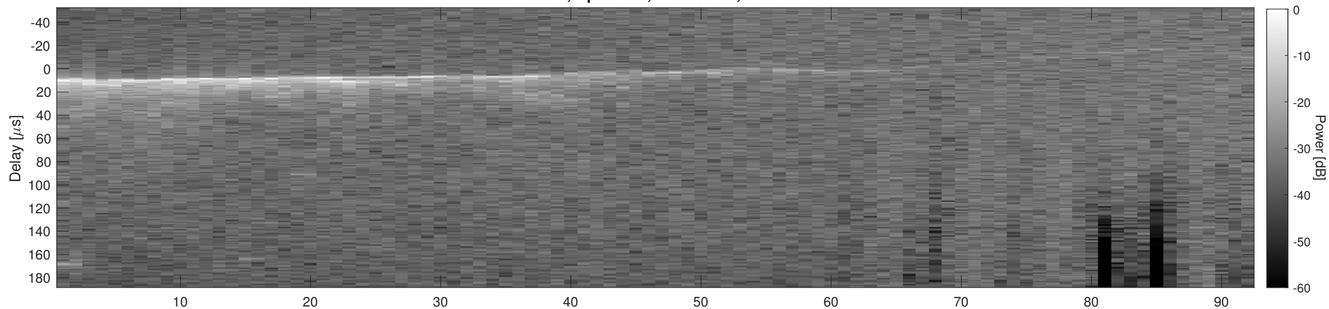
Orbit 2840, Cluttergram
