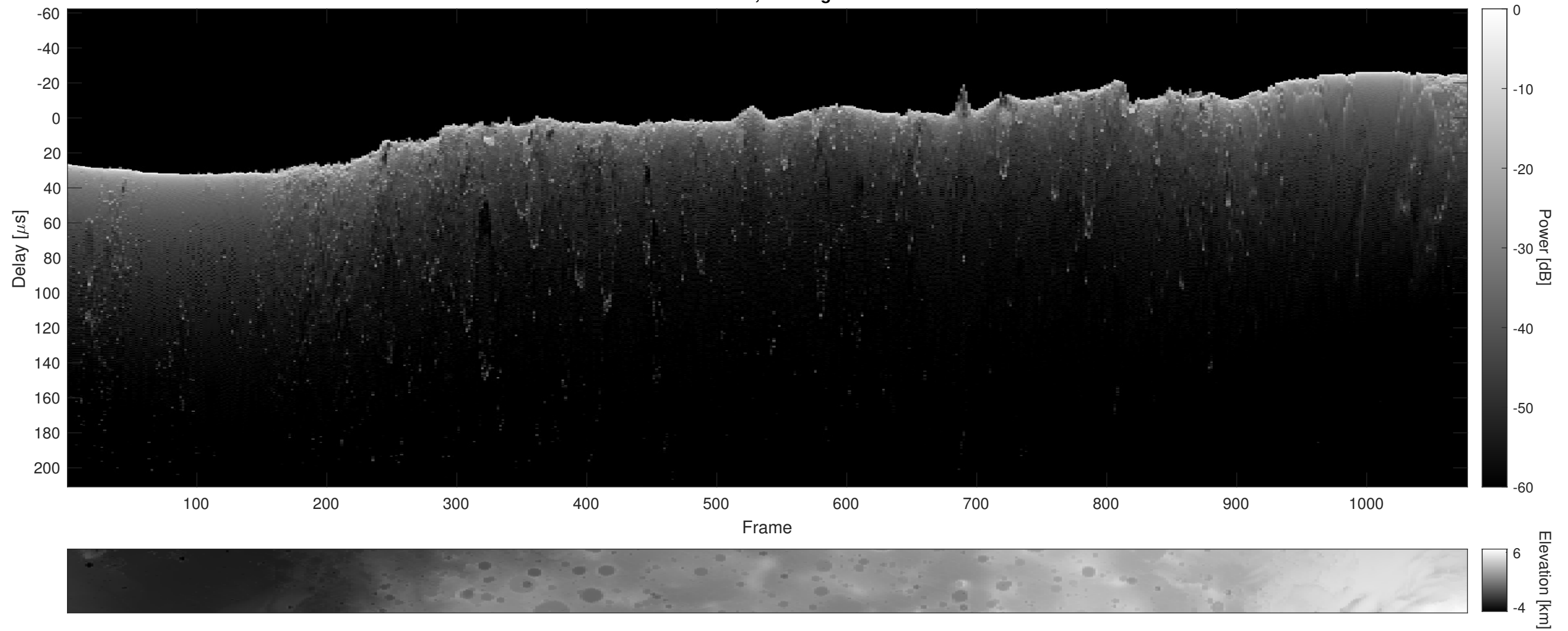
Orbit 2841, Cluttergram
