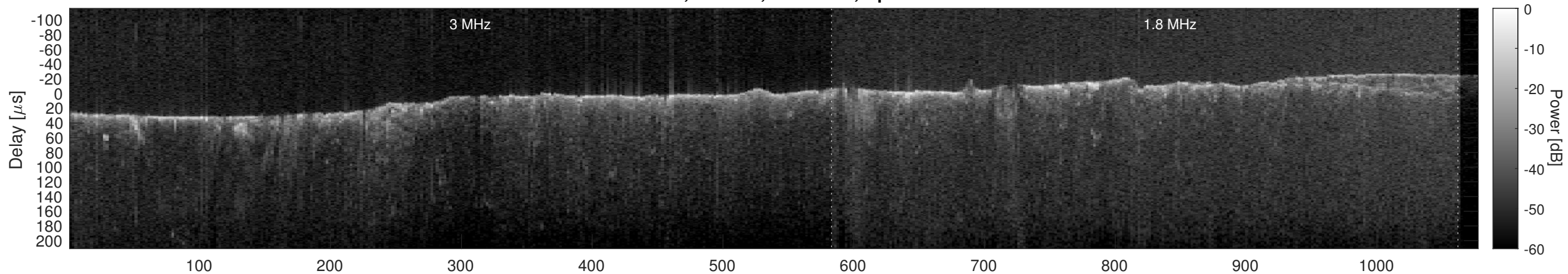
Orbit 2841, Cluttergram
