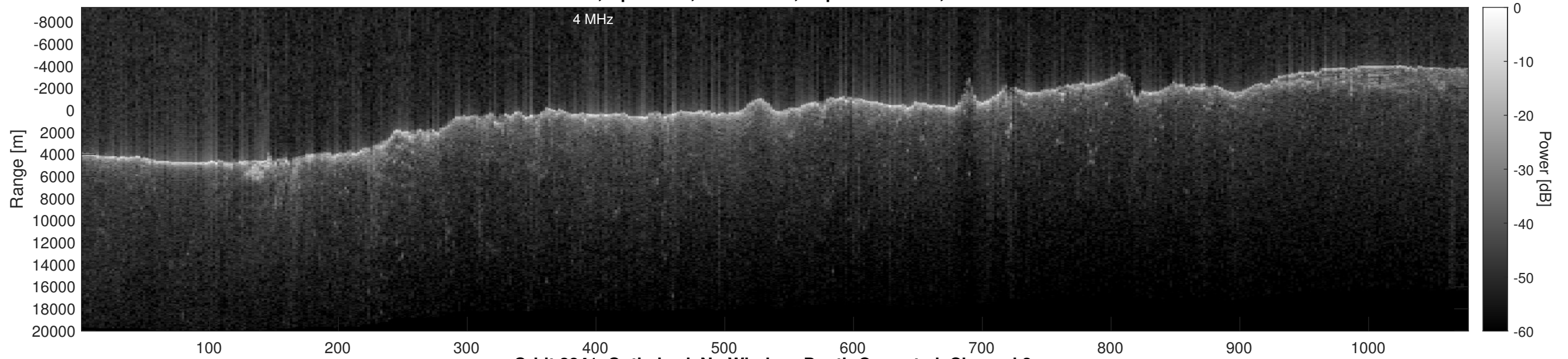
Orbit 2841, Optimized, No Window, Depth-Corrected, Channel 2
