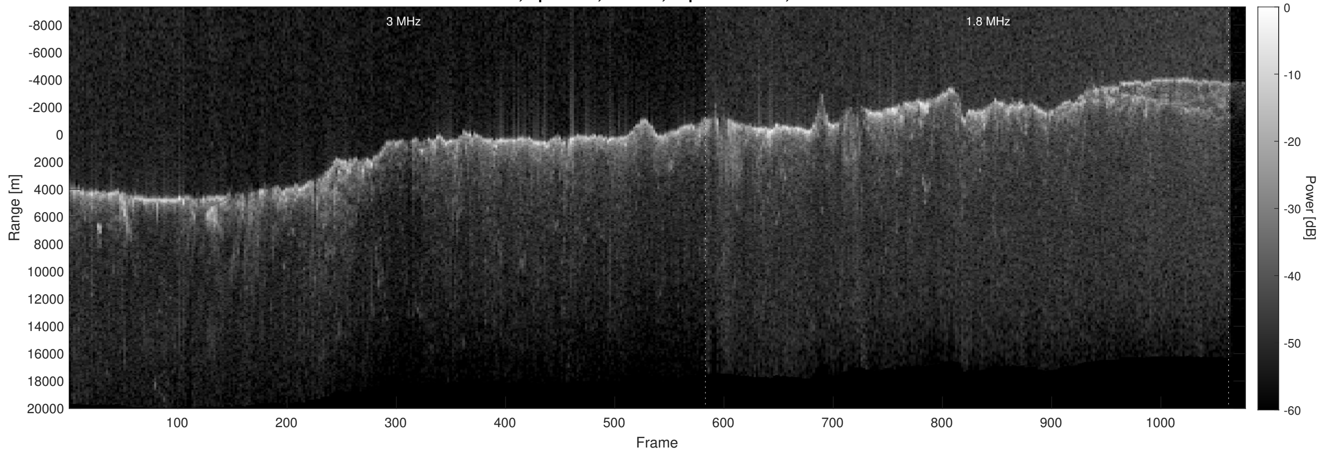
Orbit 2841, Optimized, Window, Depth-Corrected, Channel 2
