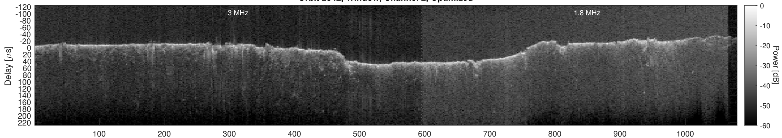
Orbit 2842, Cluttergram
