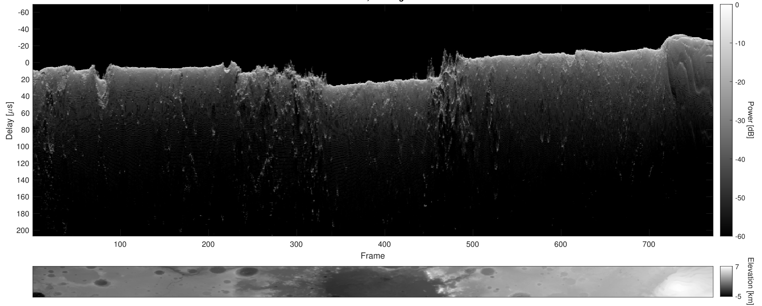
Orbit 2843, Cluttergram
