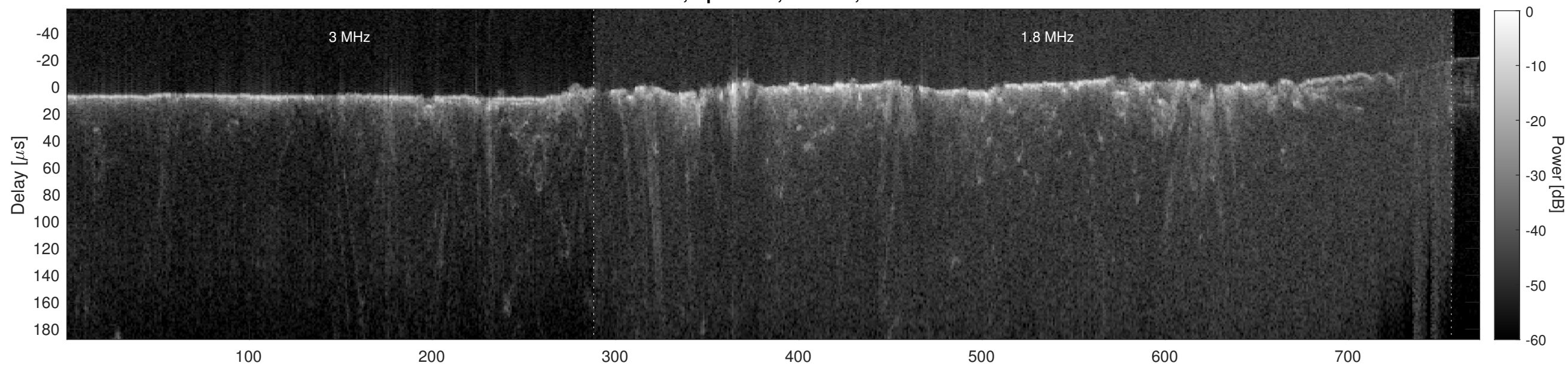
Orbit 2844, Cluttergram
