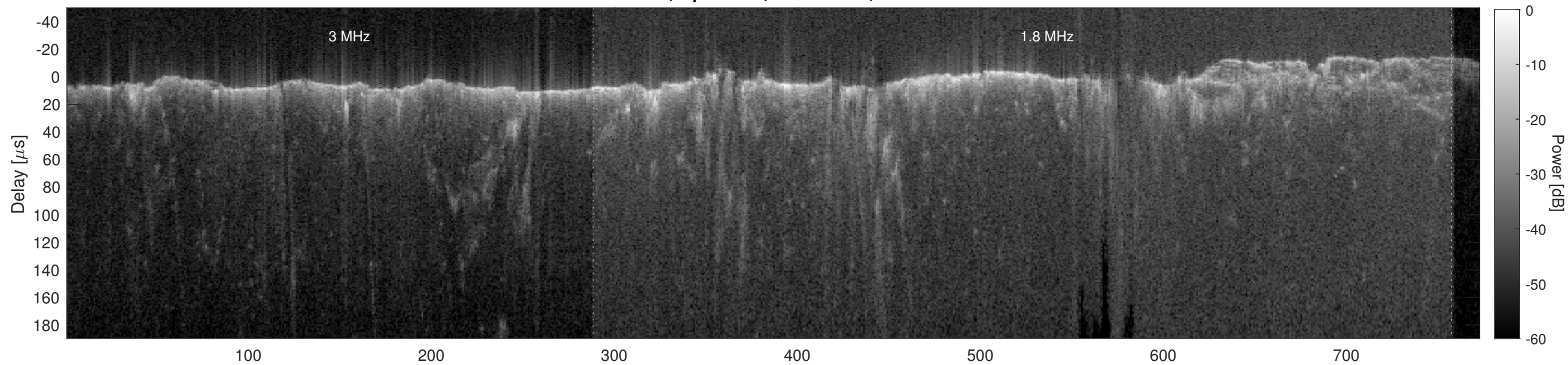
Orbit 2845, Cluttergram
