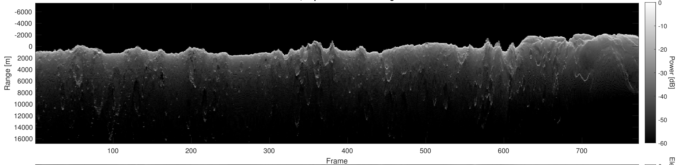
Orbit 2845, Depth-Corrected Cluttergram
