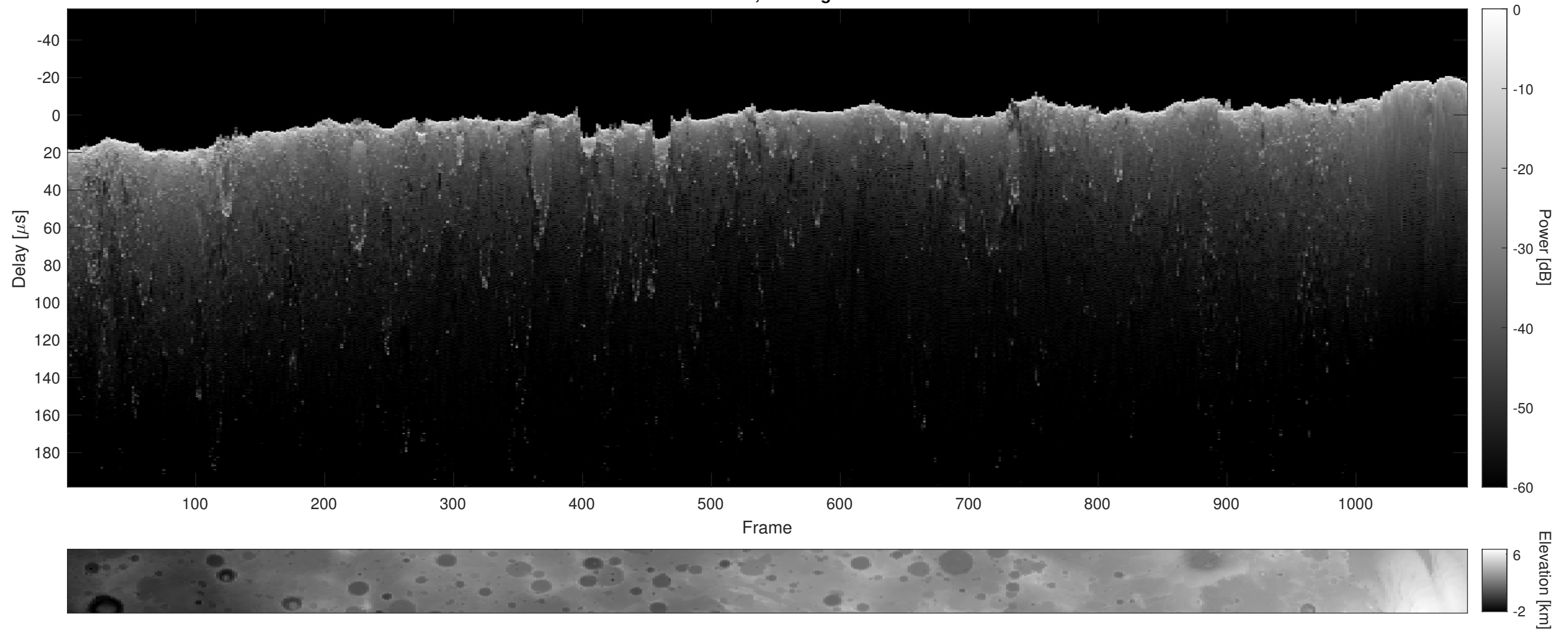
Orbit 2846, Cluttergram
