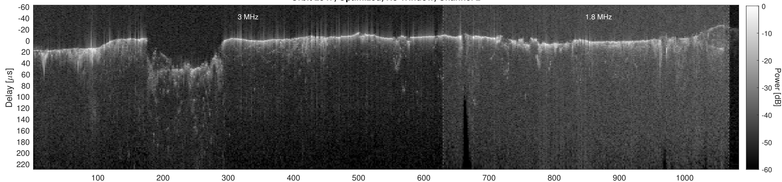
Orbit 2847, Cluttergram
