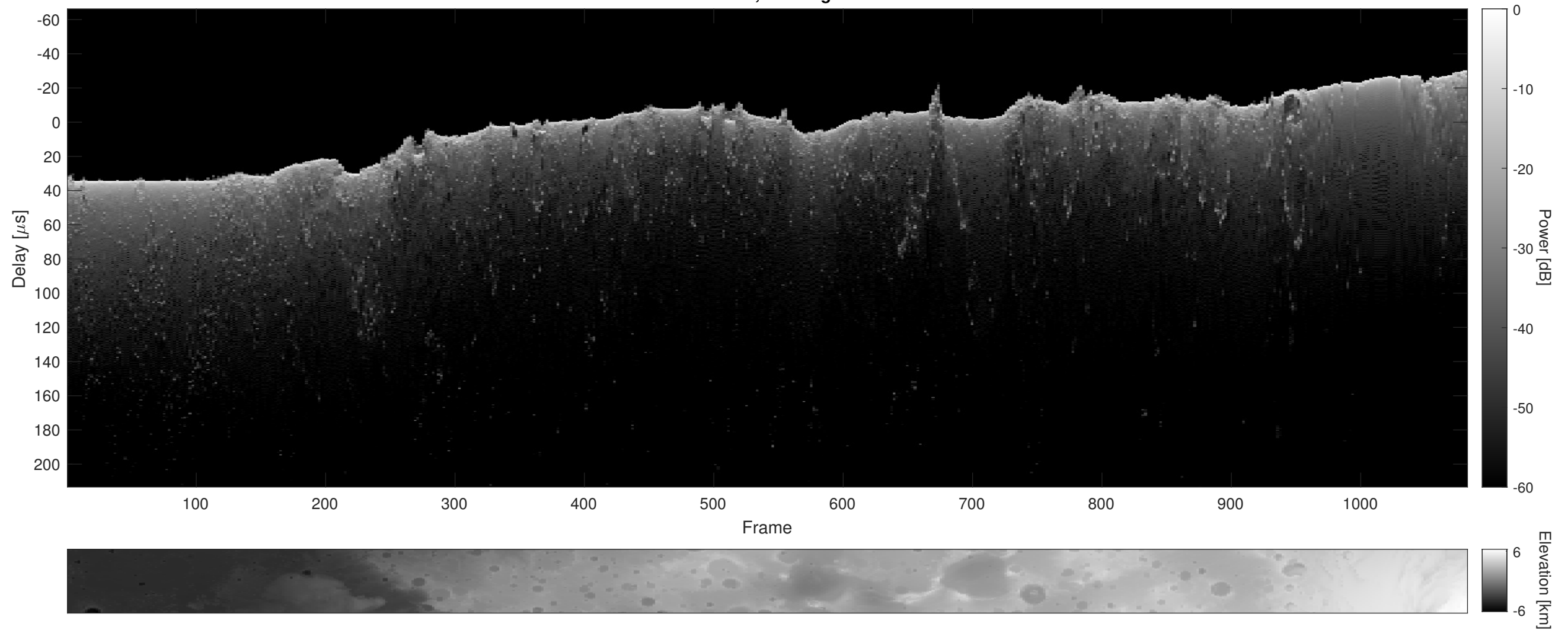
Orbit 2848, Cluttergram
