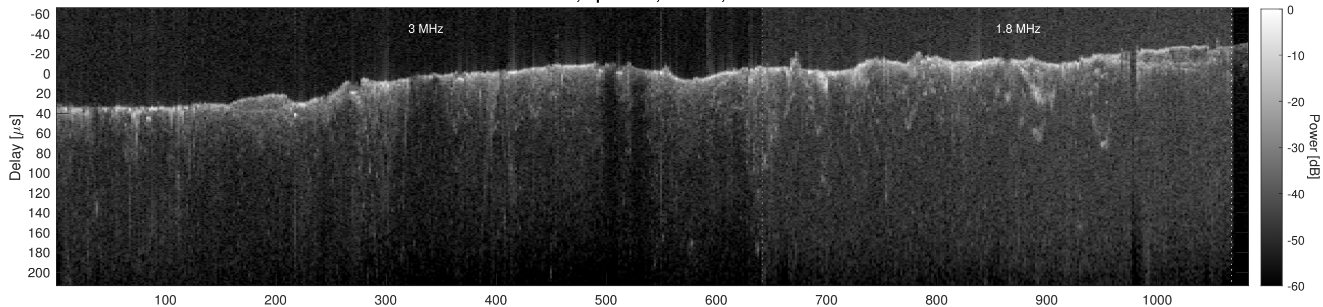
Orbit 2848, Cluttergram
