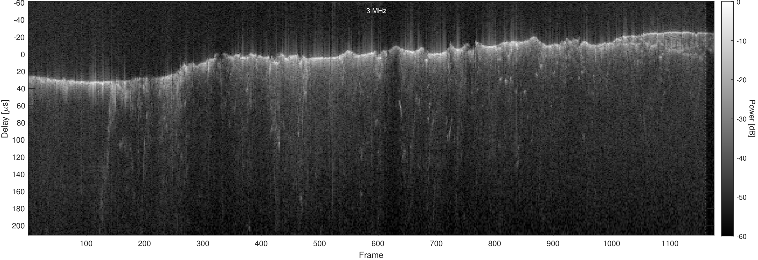
Orbit 2852, Optimized, No Window, Channel 2
