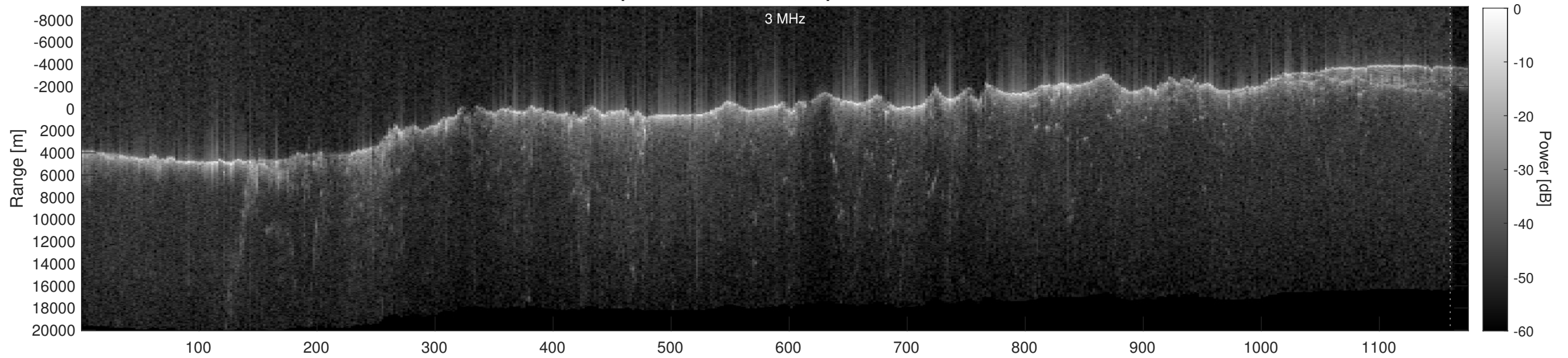
Orbit 2852, Depth-Corrected Cluttergram
