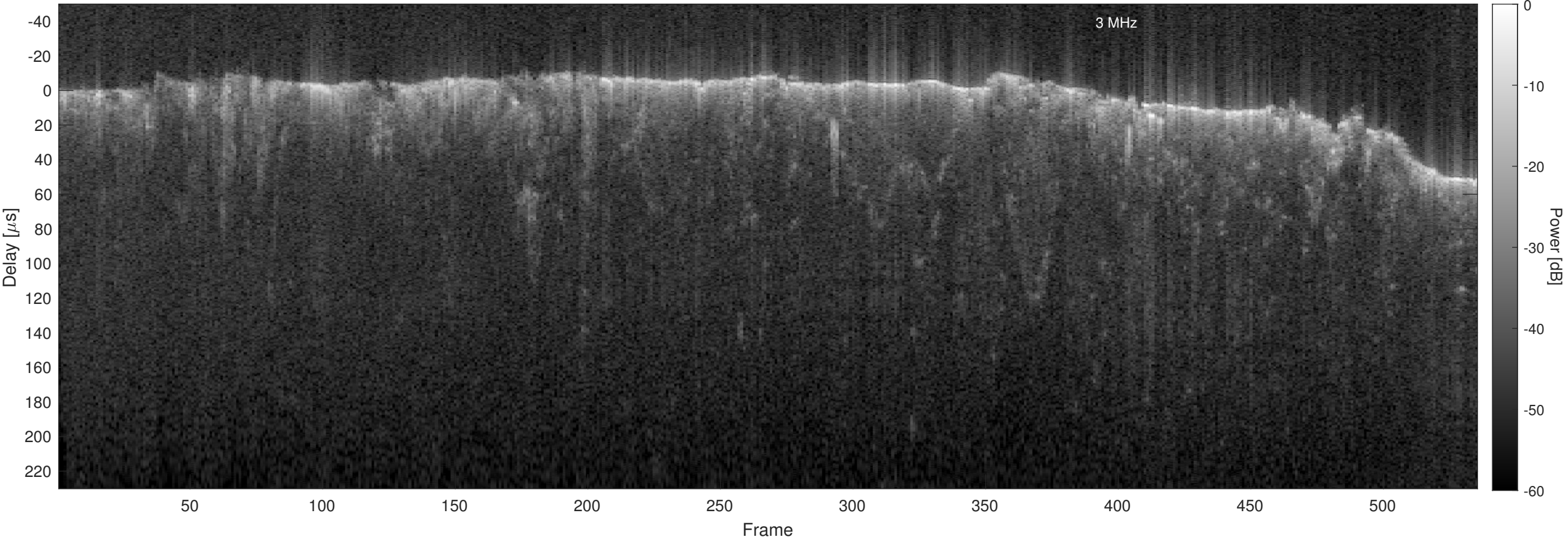
Orbit 2853, Optimized, No Window, Channel 2
