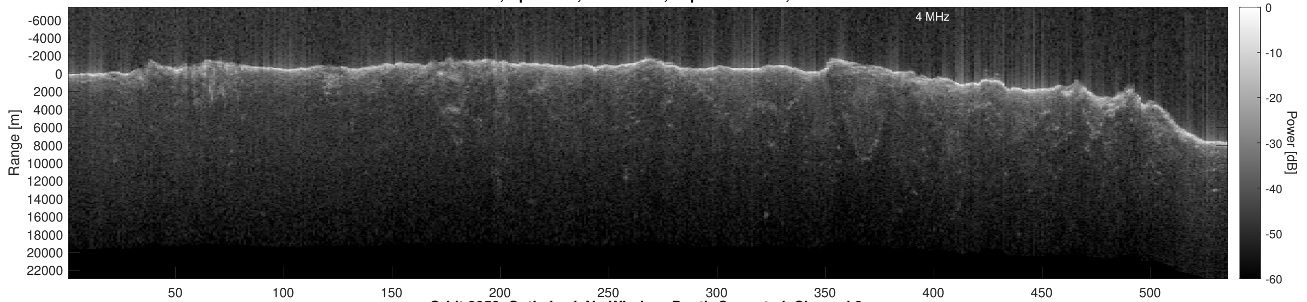
Orbit 2853, Optimized, No Window, Depth-Corrected, Channel 2
