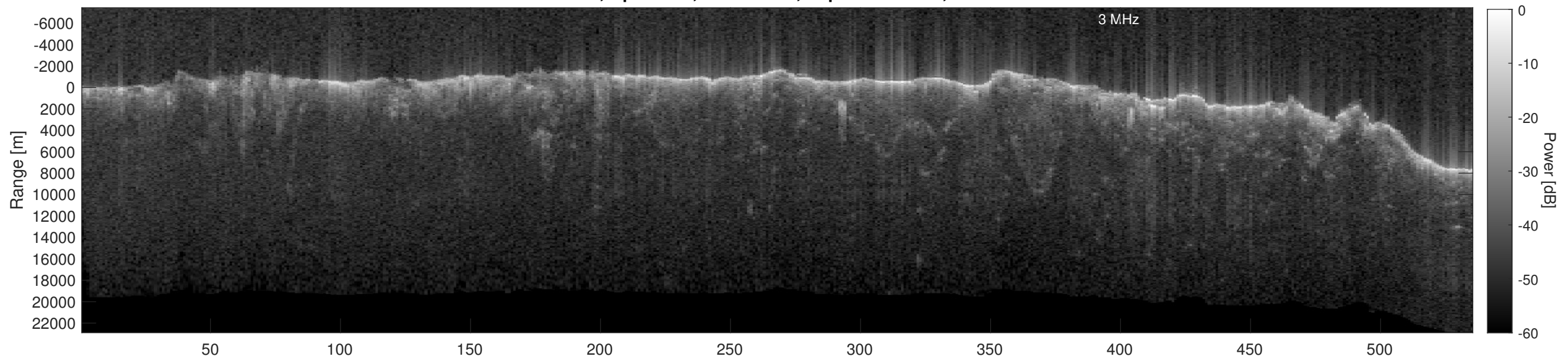
Orbit 2853, Depth-Corrected Cluttergram
